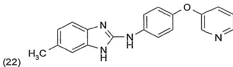
(6-Methyl-1H-benzimidazol-2-yl)-[4-(pyridin-3-yloxy)-phenyl]-amin
